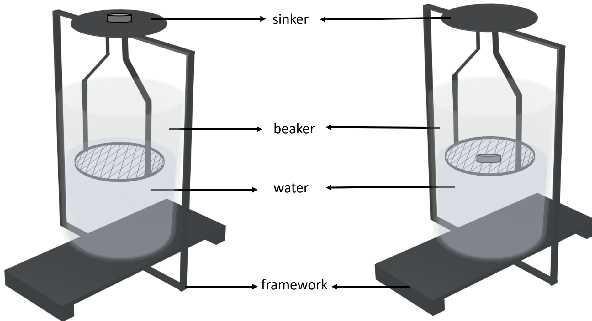
(A) Measurement setup for m_{air}
